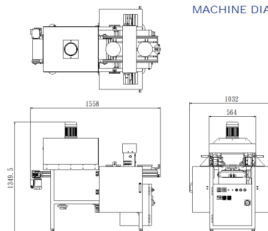
MACHINE DIAGRAM
